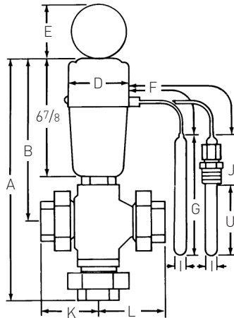
Three-way Valve
