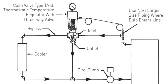
Figure 6 - Type TA 3-Way Used As A Diverting Valve (Flow travels in opposite direction of arrow cast on body.)
