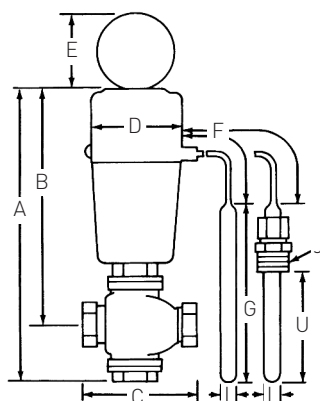
Double-Seated Reverse Acting Bronze Valve
