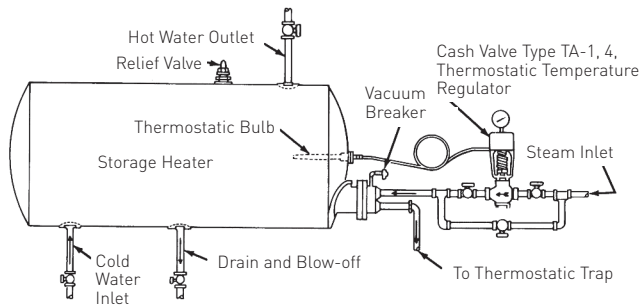
Figure 1 - Controlling Storage Heater
