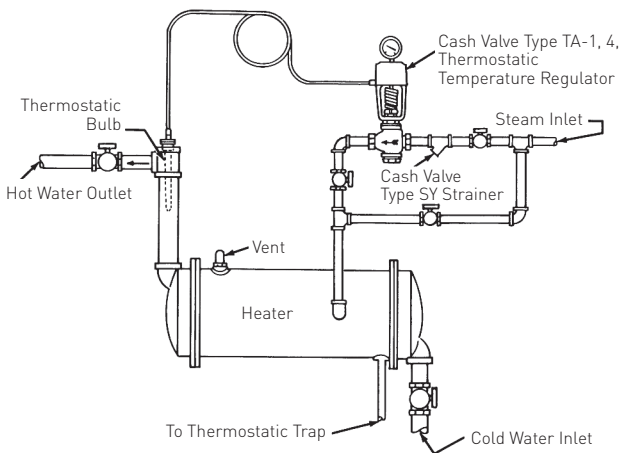
Figure 3 - Controlling Instantaneous Water Heater
